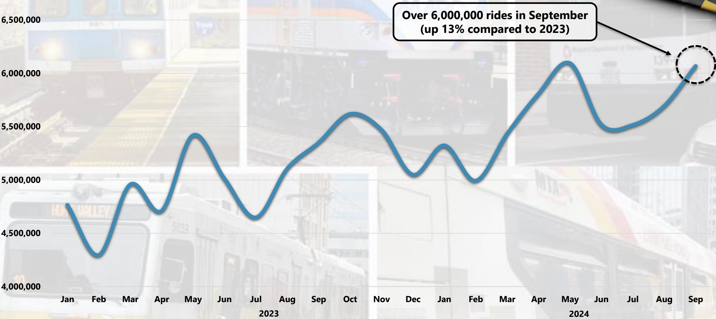
Total MTA Ridership by Month
